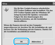
Windows XP
