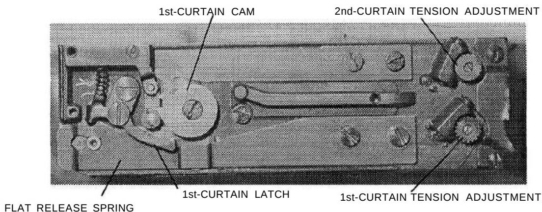
FIG. L3 BOTTOM OF CAMERA, SHUTTER RELEASED
