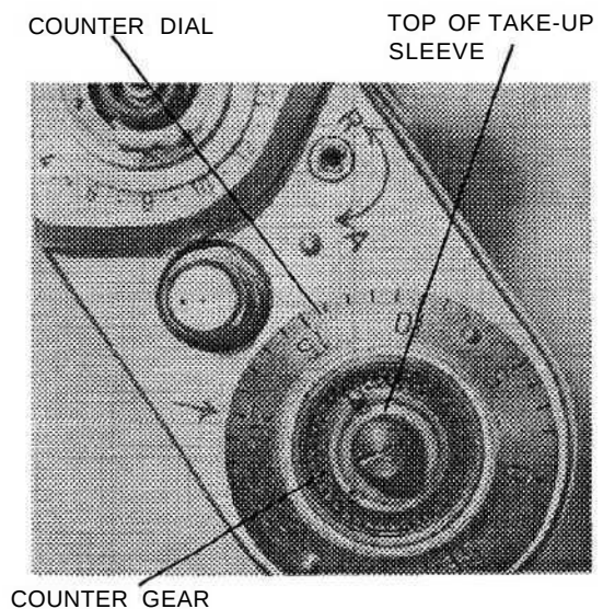
FIG. L18 Top, wind knob removed.
