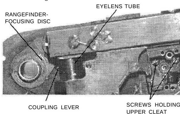
FIG. L40 Top view, rewind end.
