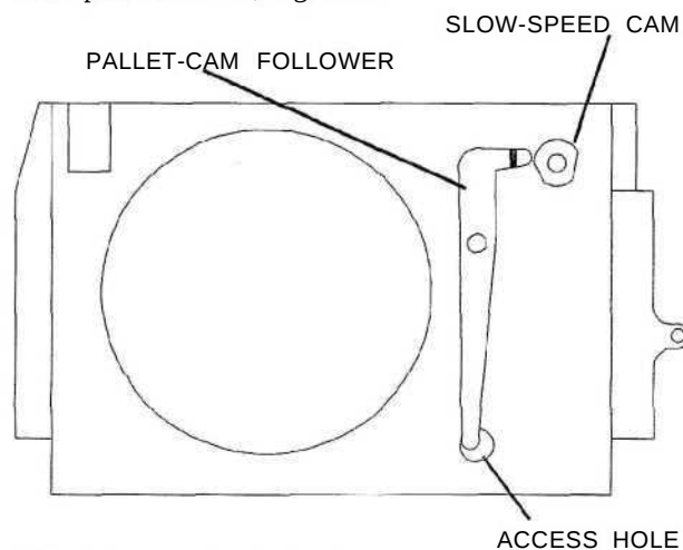
FIG. L36 Back of the front plate.
