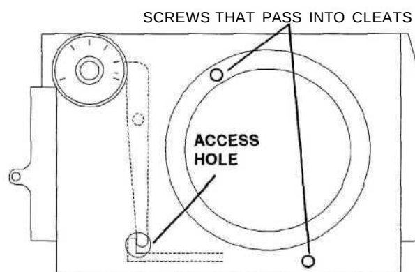
FIG. L42 Connection between the pallet-cam follower and the pallet lever.
