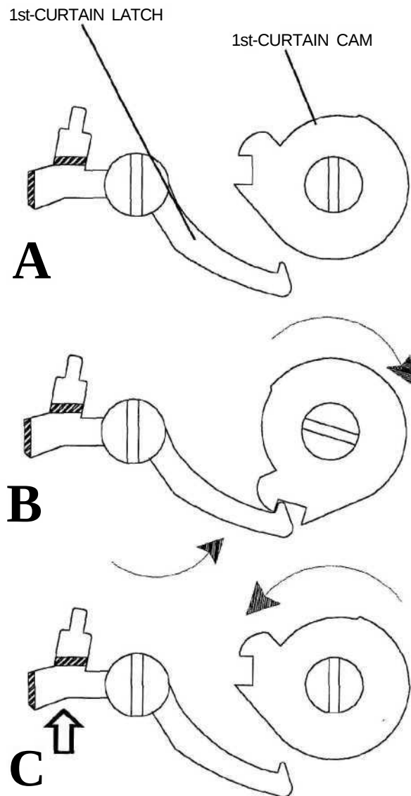
FIG. L6 Sequence of the 1st-curtain release action. In A, the shutter is in the released position. As you cock the shutter, the 1st-curtain cam turns clockwise; the 1st-curtain latch then latches the 1st-curtain cam (B). In C, the flat release spring has disengaged the 1st-curtain latch. The 1st-curtain now rotates counterclockwise as the 1st curtain crosses the film aperture.
