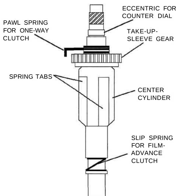
FIG. L21 Take-up sleeve removed from camera.
