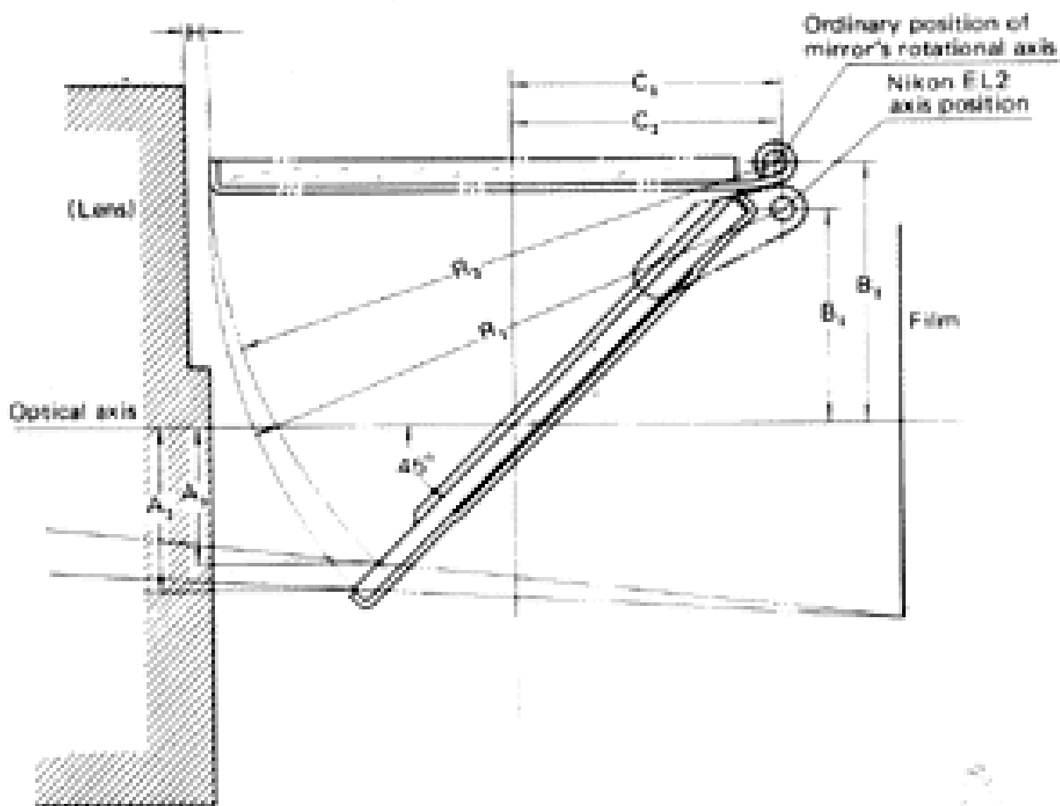
Mirror geometry
