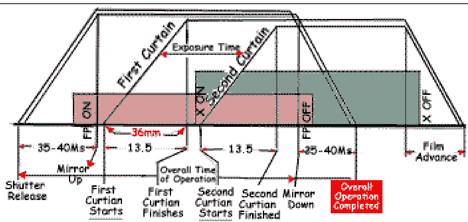
Shutter Timing of the Olympus OM-1(n)
