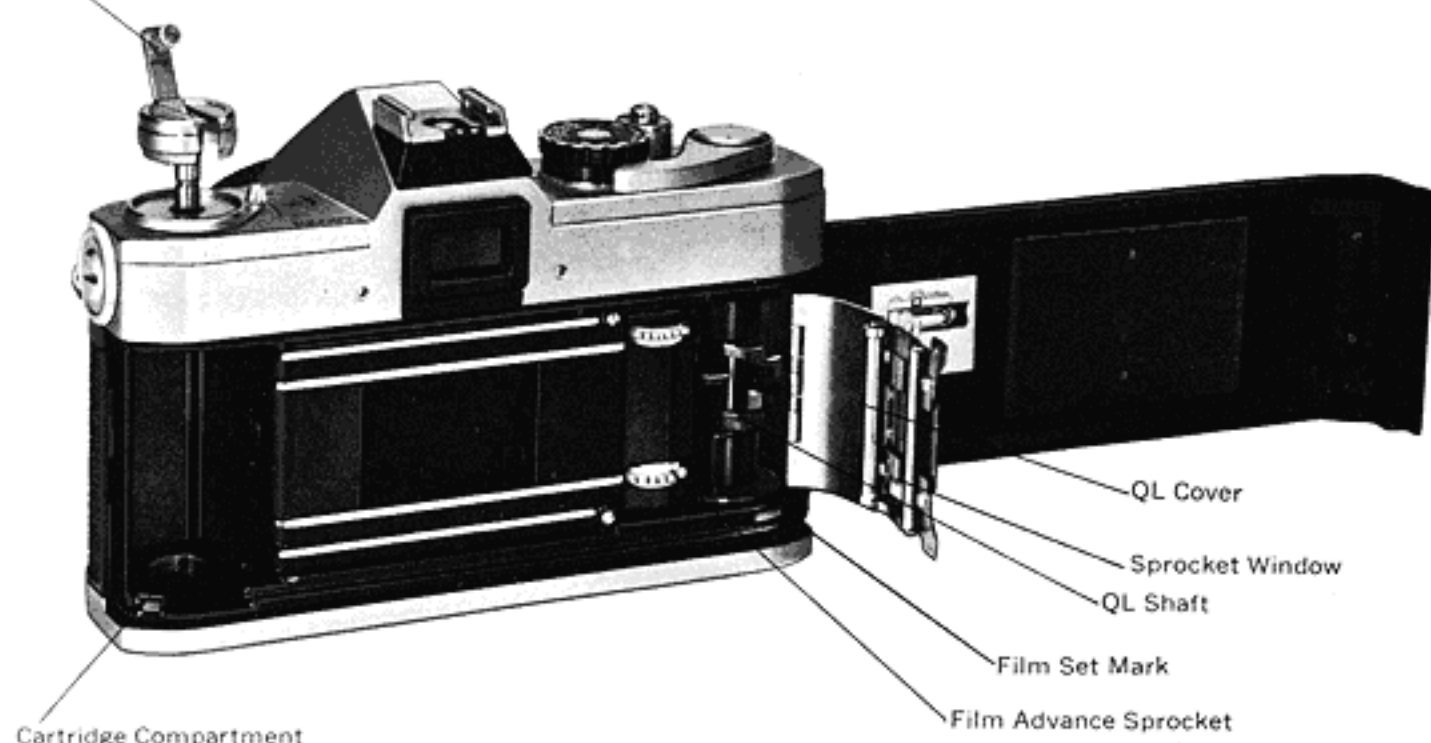
Film Rewinding Crank
