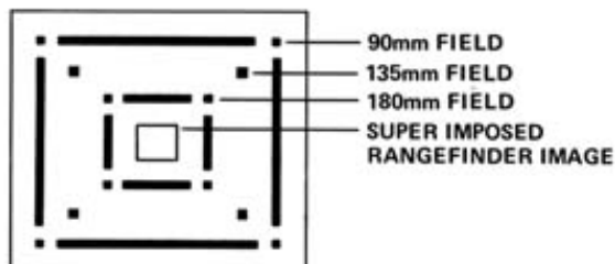
Viewfinder Window
