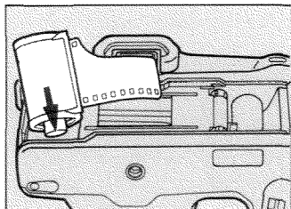
4. Load film (p. 13)
