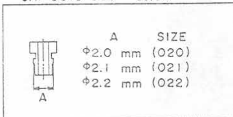
CAI-6616-000 detail
