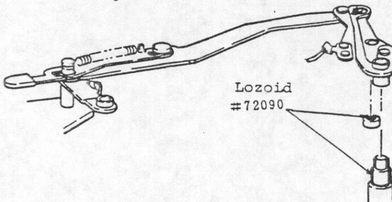
Connecting Lever
