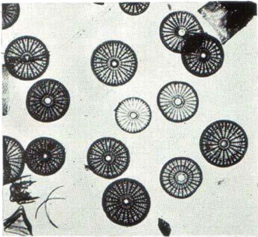
Photomicrographed diatoms on spider web.
