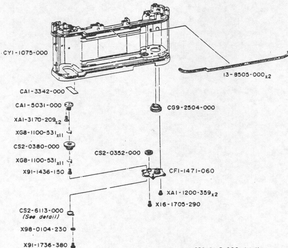
CS2-6113-000 detail
