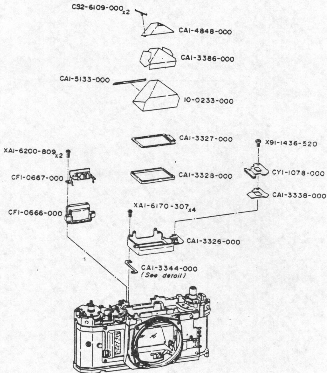
CAI-3344-000 detail
