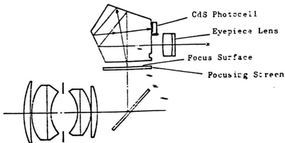
Figure 5: Optical Schematic of AF-1 with PD 50mm 1:1.3 S.C.
