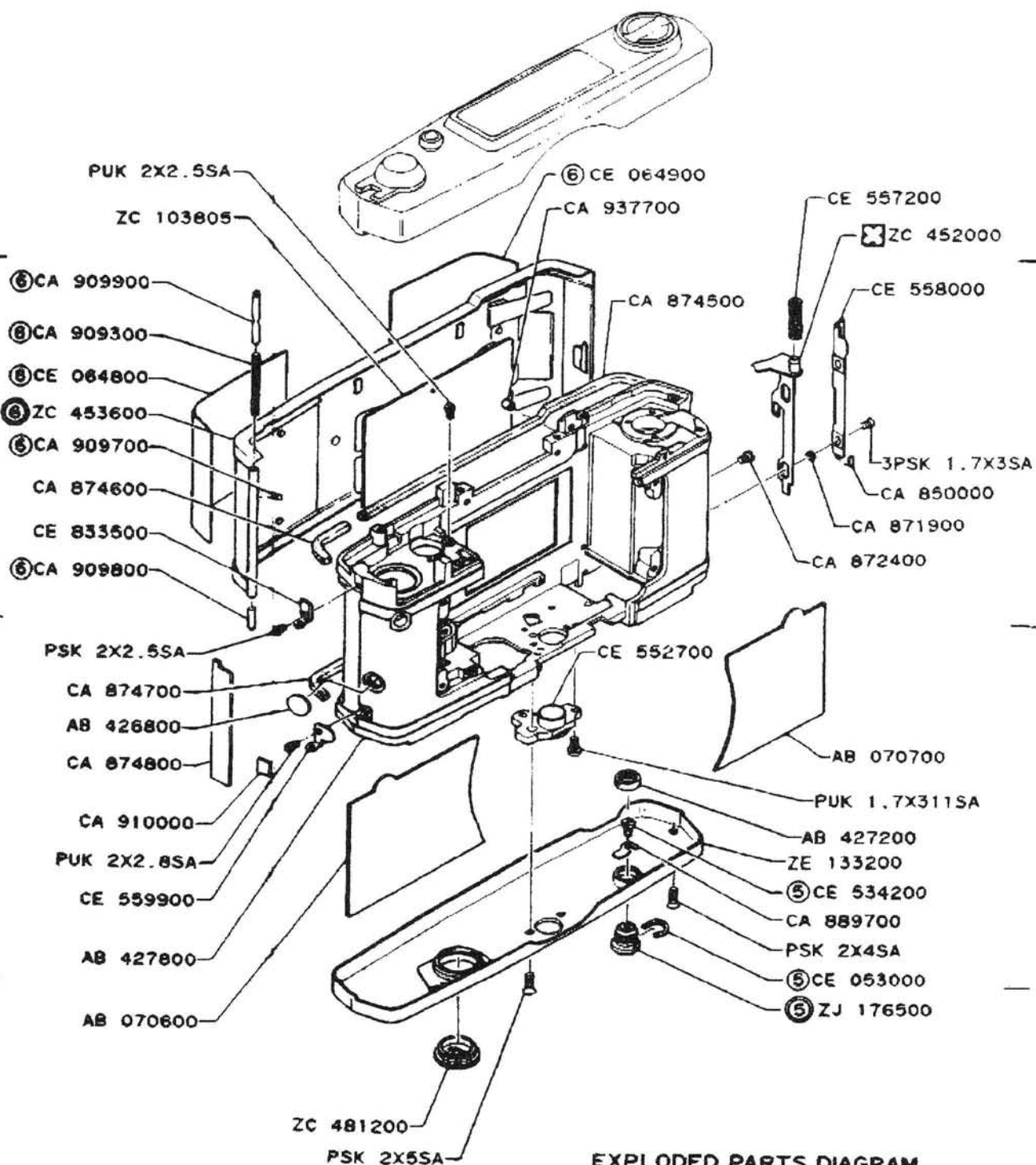
EXPLODED PARTS DIAGRAM
