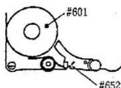
Hooking position of spring #652
