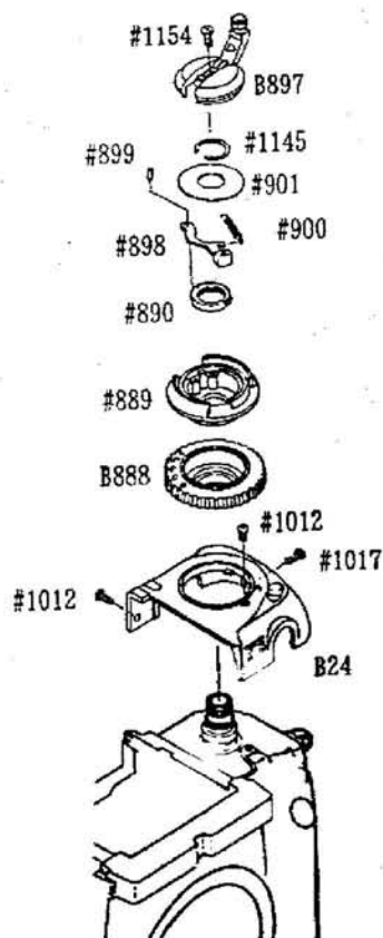
Top cover on film rewind side
