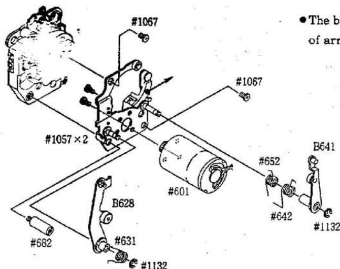
Hooking position of spring #631
