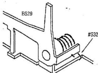
Hooking position of spring #532
