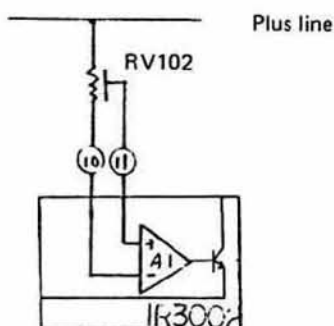
The lock voltage of 2.2 \pm 0.05 V is adjusted by RV102.
