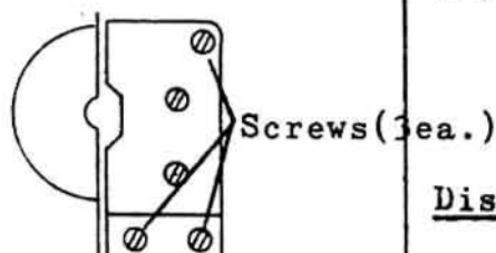
Shutter Spring Axle Holder
