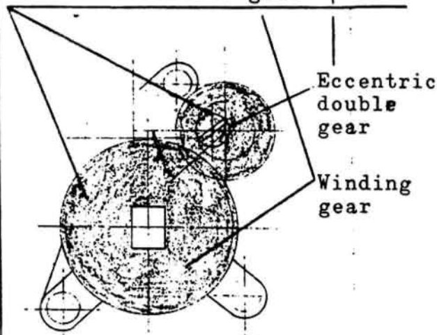
Relation of the square opening and the eccentric gear
