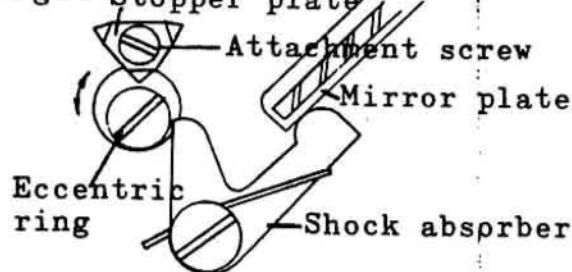
Fig.4 Stopper plate
