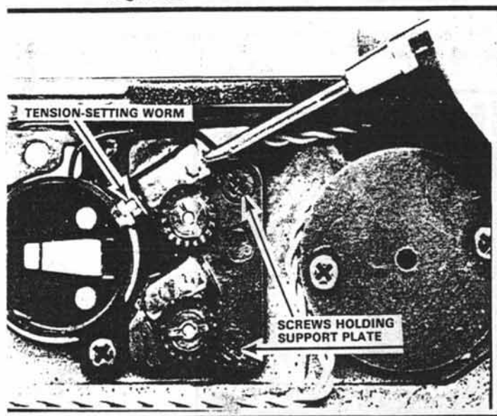
Figure 166 Removing the closing-curtain tension-setting worm
