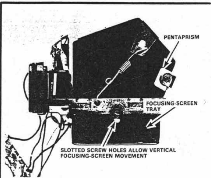
Figure 79 Assembly with pentaprism in place.
