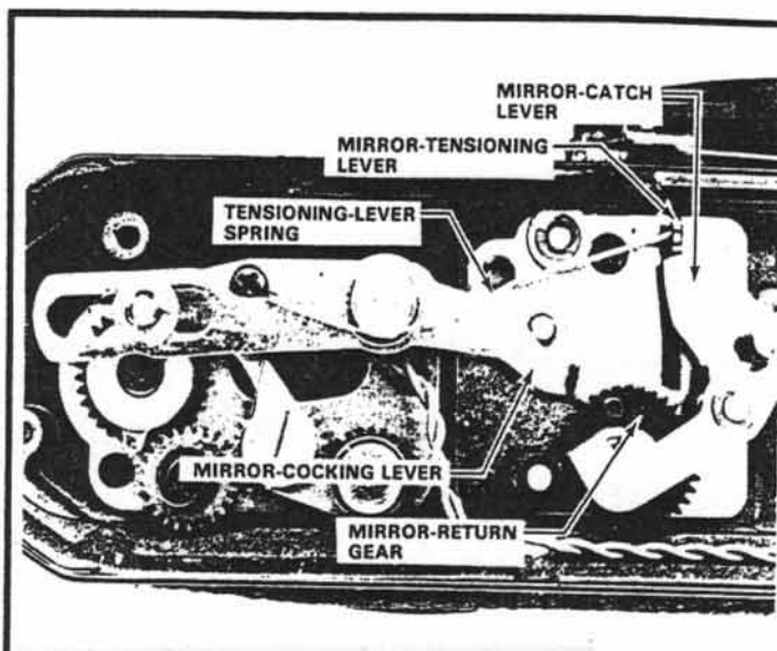
Figure 88 Shutter cocked
