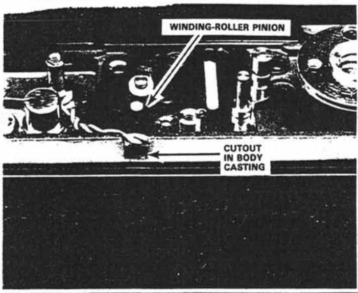
Figure 155 Shutter released
