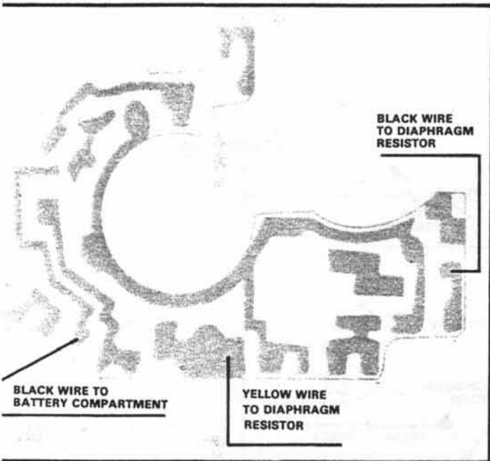
Figure 75 Exposure-meter circuit board
