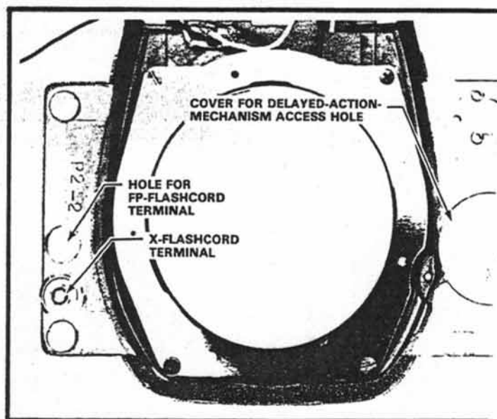
Figure 86 Back of front standard
