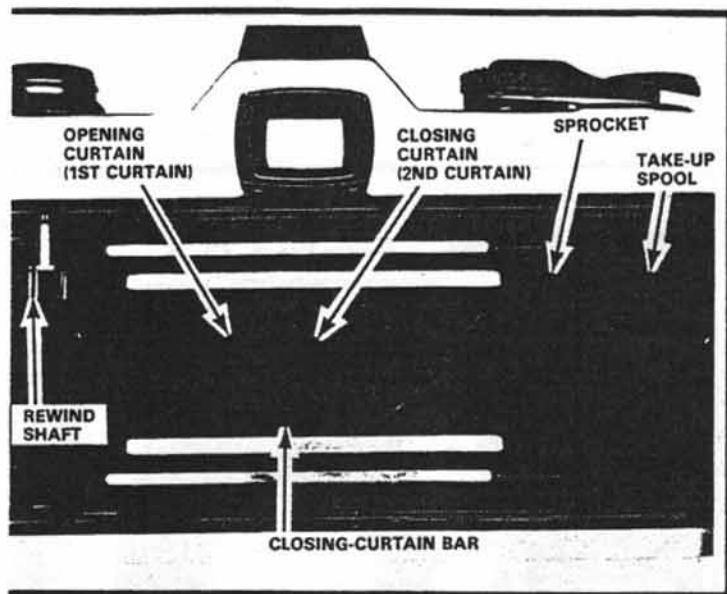
Figure 8 Curtain movement during cocking cycle
