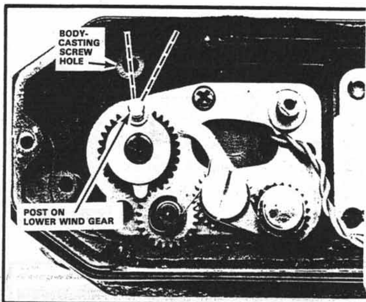
Figure 199 Tolerance- Post can be 10° to right of screw hole
