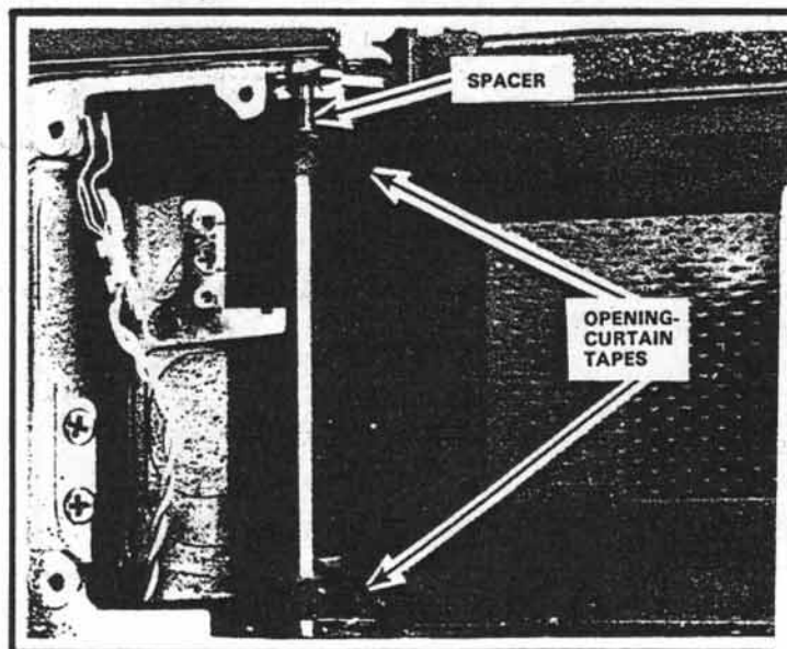
Figure 173 Opening-curtain winding roller installed
