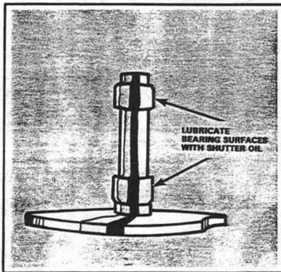
Figure 207 Release cam
