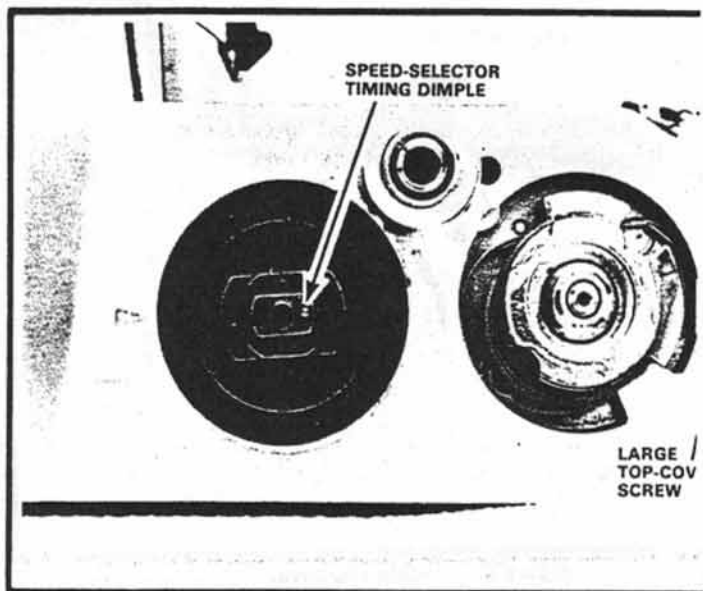
Figure 28 Bulb setting
