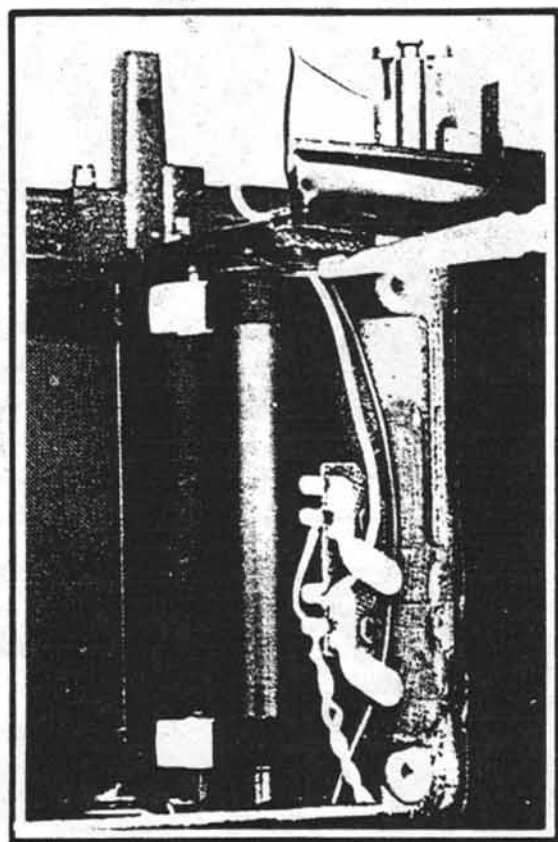
Figure 150 Using an artist-type brush to apply cleaning solution to the take-up-rollers' bearings.
