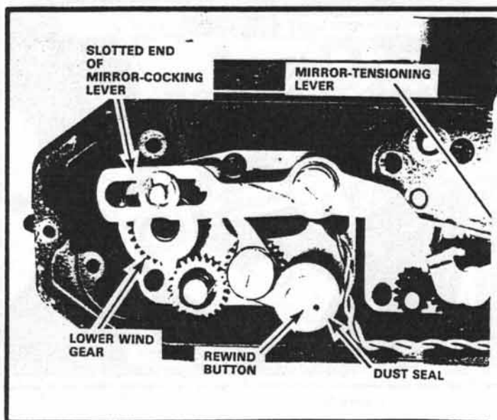
Figure 11 Shutter released
