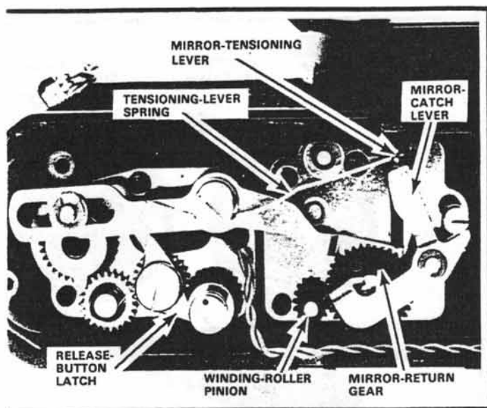
Figure 12 Shutter cocked
