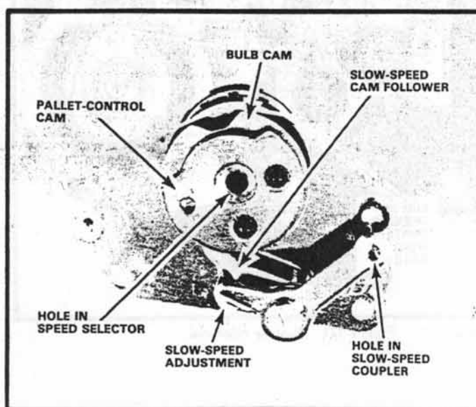
Figure 119 Bottom of speed selector
