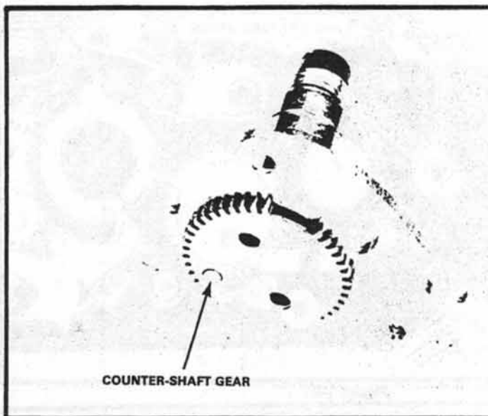
Figure 137 Bottom of support-shaft assembly 03239 03339
