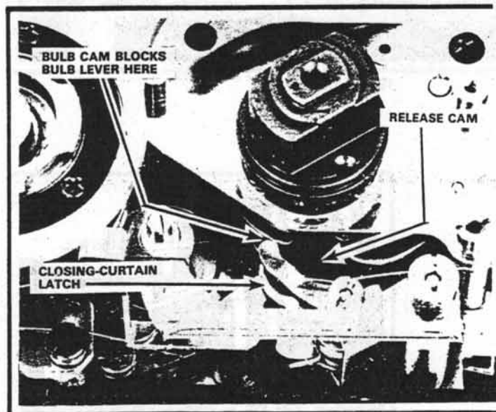
Figure 109 1-second setting
