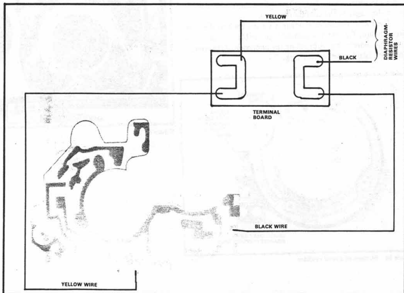
Figure 56 Exposure-meter circuit board
