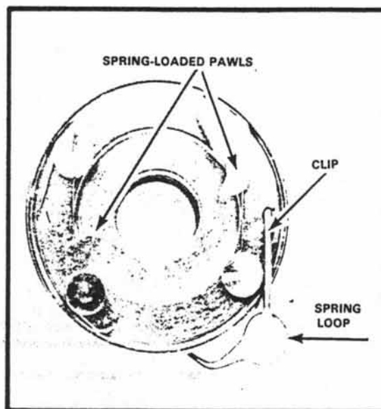
Figure 131 Bottom of wind driver
