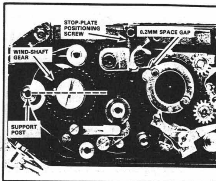
Figure 198 Shutter cocked
