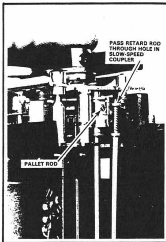
Figure 208 Seating the speed-selector assembly
