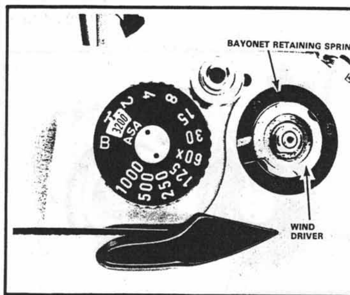
Figure 21 The three raised lugs of the bayonet retaining spring go up.
