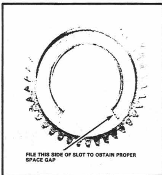
Figure 204 Upper transport gear
