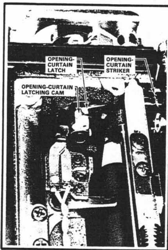
Figure 87 Shutter cocked
