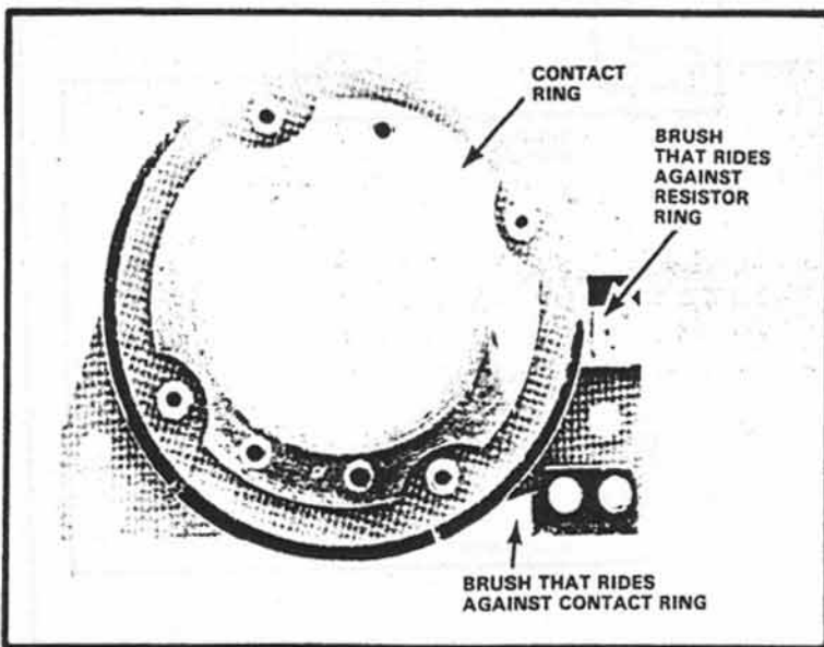
Figure 54 Bottom of speed resistor
