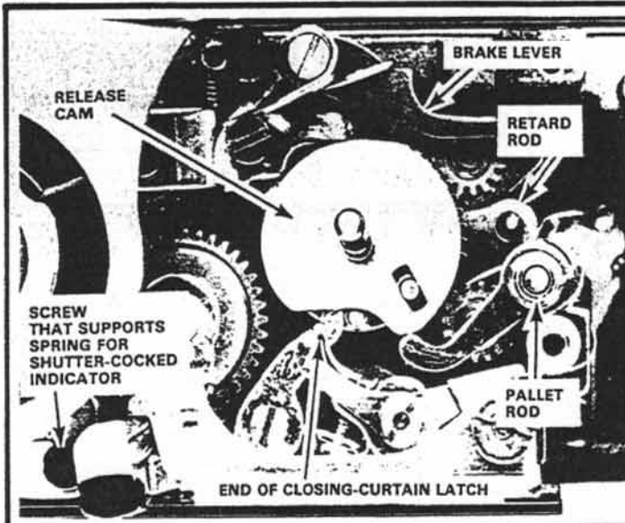
Figure 206 Shutter cocked
