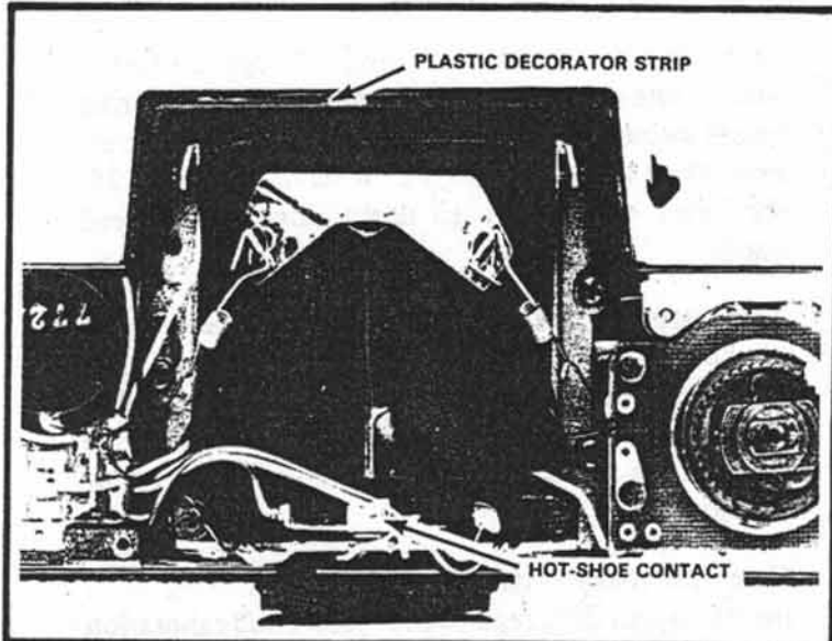
Figure 31 The hot-shoe contact engages a contact in the top-cover accessory shoe.
