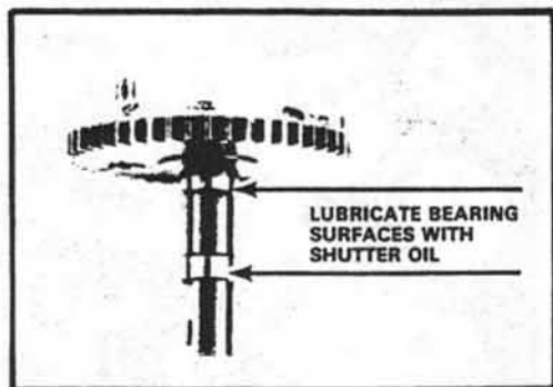
Figure 181 Opening-curtain wind gear
