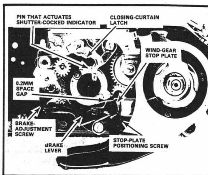
Figure 122 Shutter cocked
