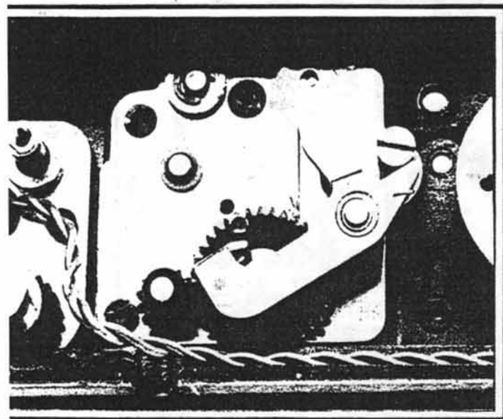
Figure 197 Shutter cocked
