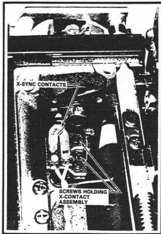
Figure 82 Shutter Released
