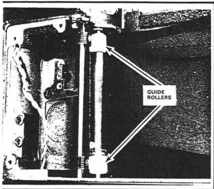
Figure 174 Closing-curtain winding roller installed
