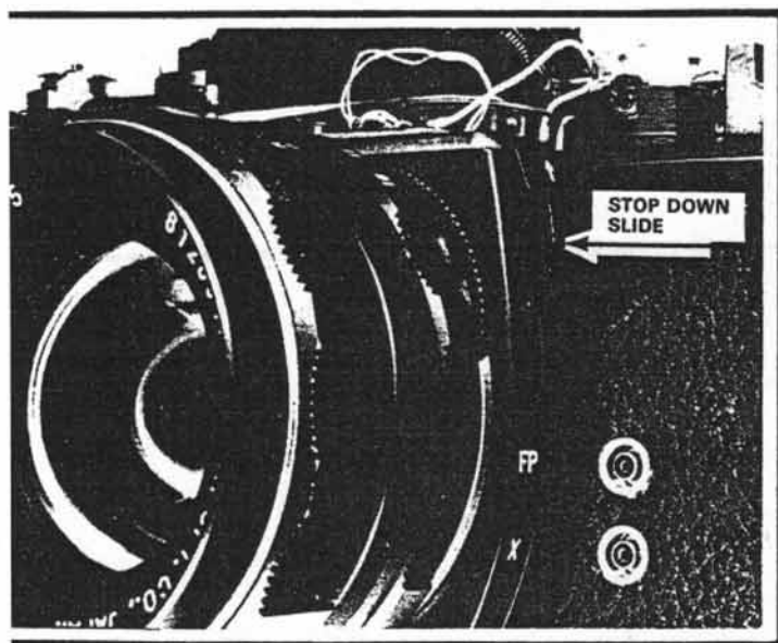
Figure 72 Spotmatic F
