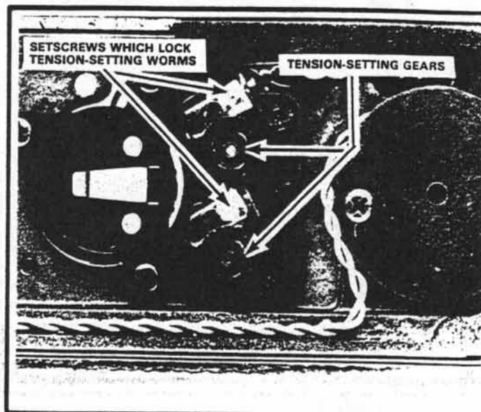
Figure 162 The tension-setting worms will be loose once you let off the initial tensions.
