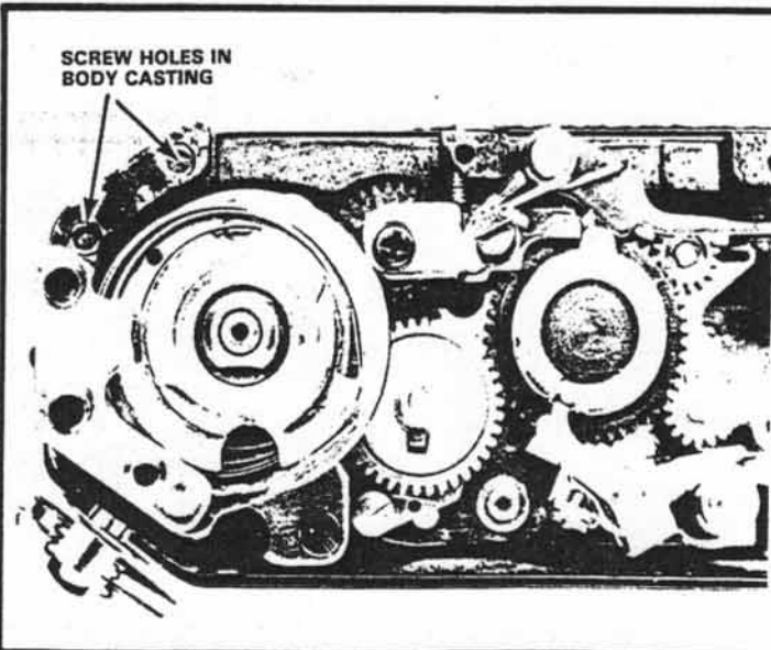
Figure 133 Starting position for replacing wind driver
