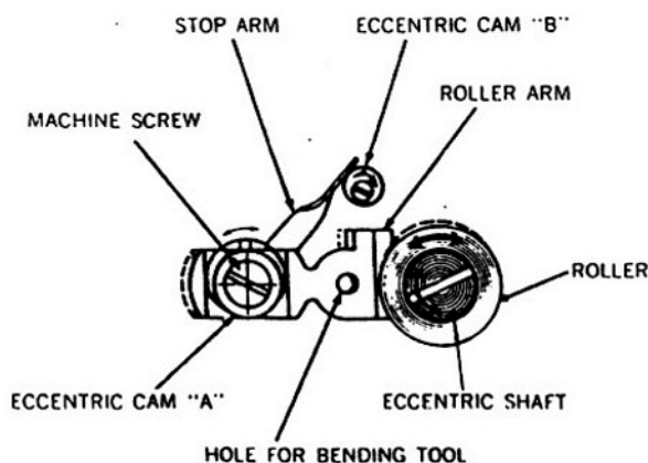
Figure 4-27. Range-Viewfinder Roller Arm.
