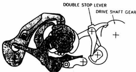
Figure 4-6. Double Stop Lever, Wound Position (Top rear view).
