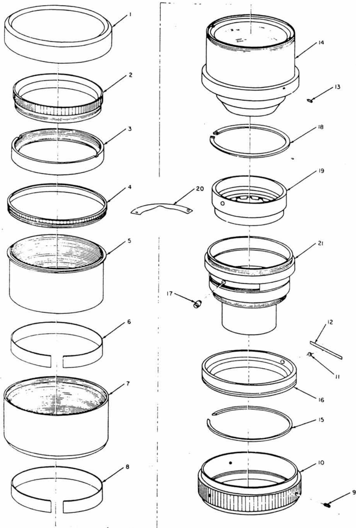
Figure 46. 135mm Lens Head (Less Optical Components), Exploded View.
