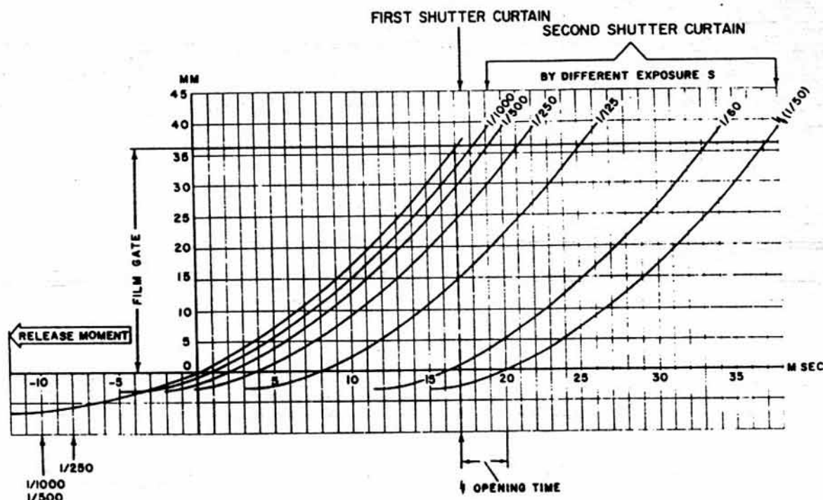
Figure 1-1. Shutter Functioning.
