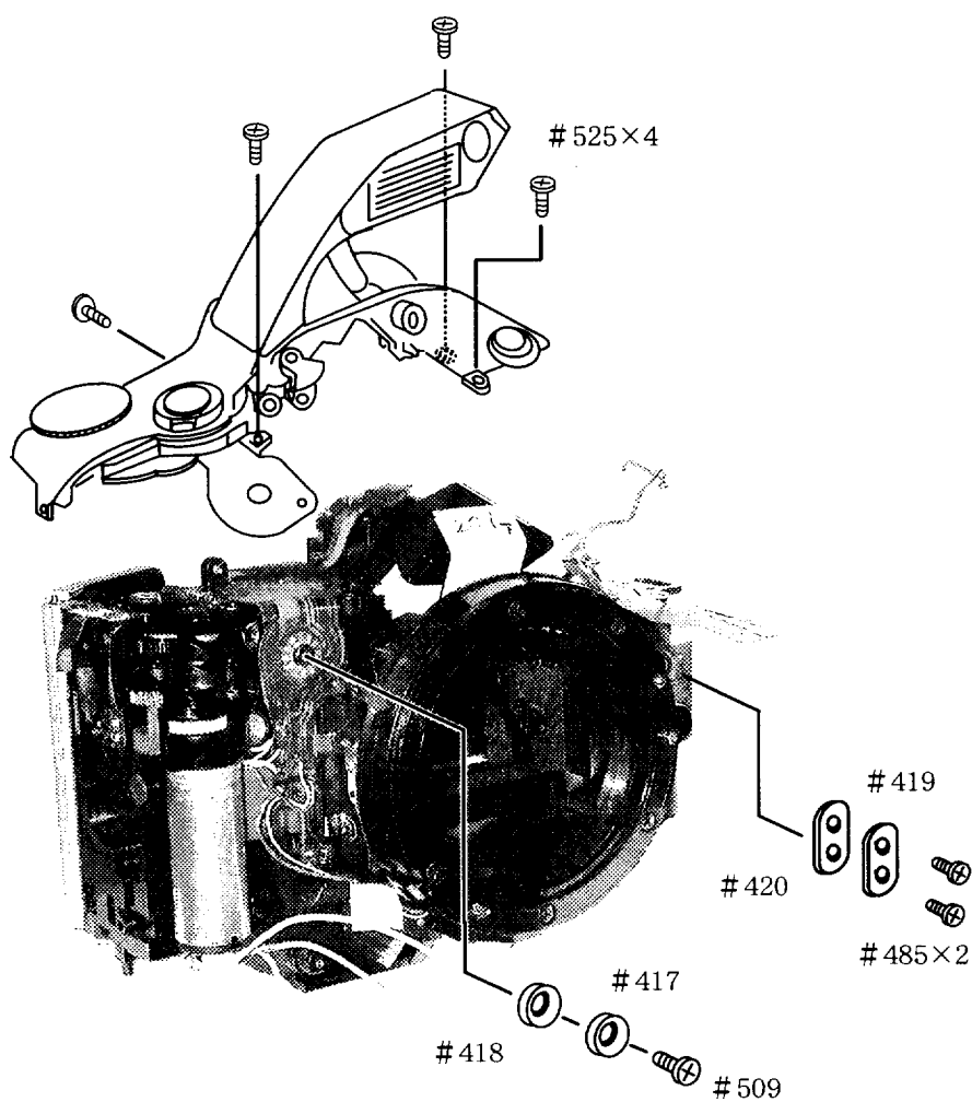
Top cover unit
