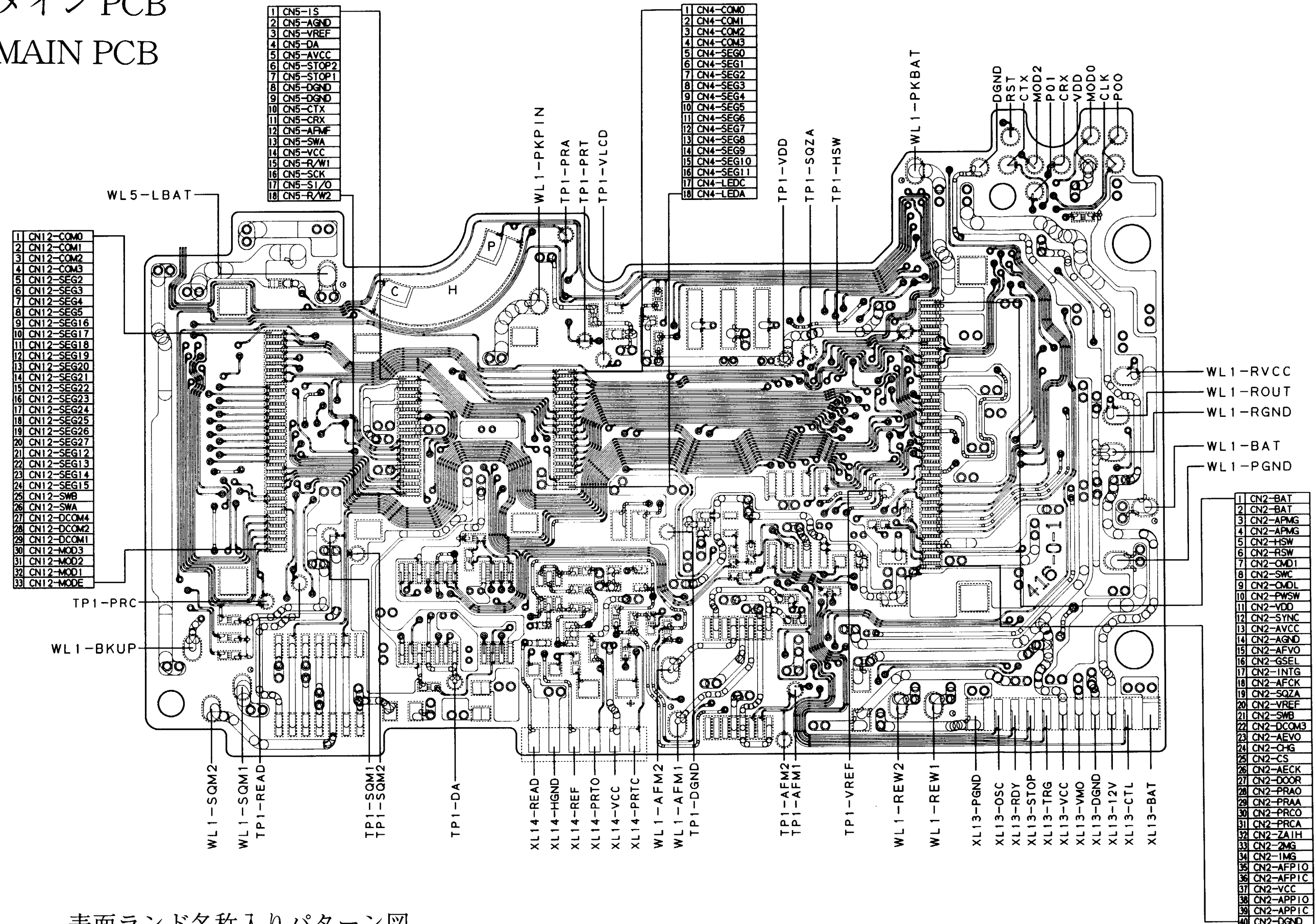
Front side pattern diagram with land name
