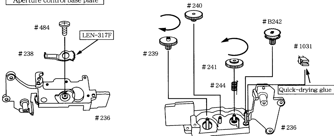
Aperture control base plate
