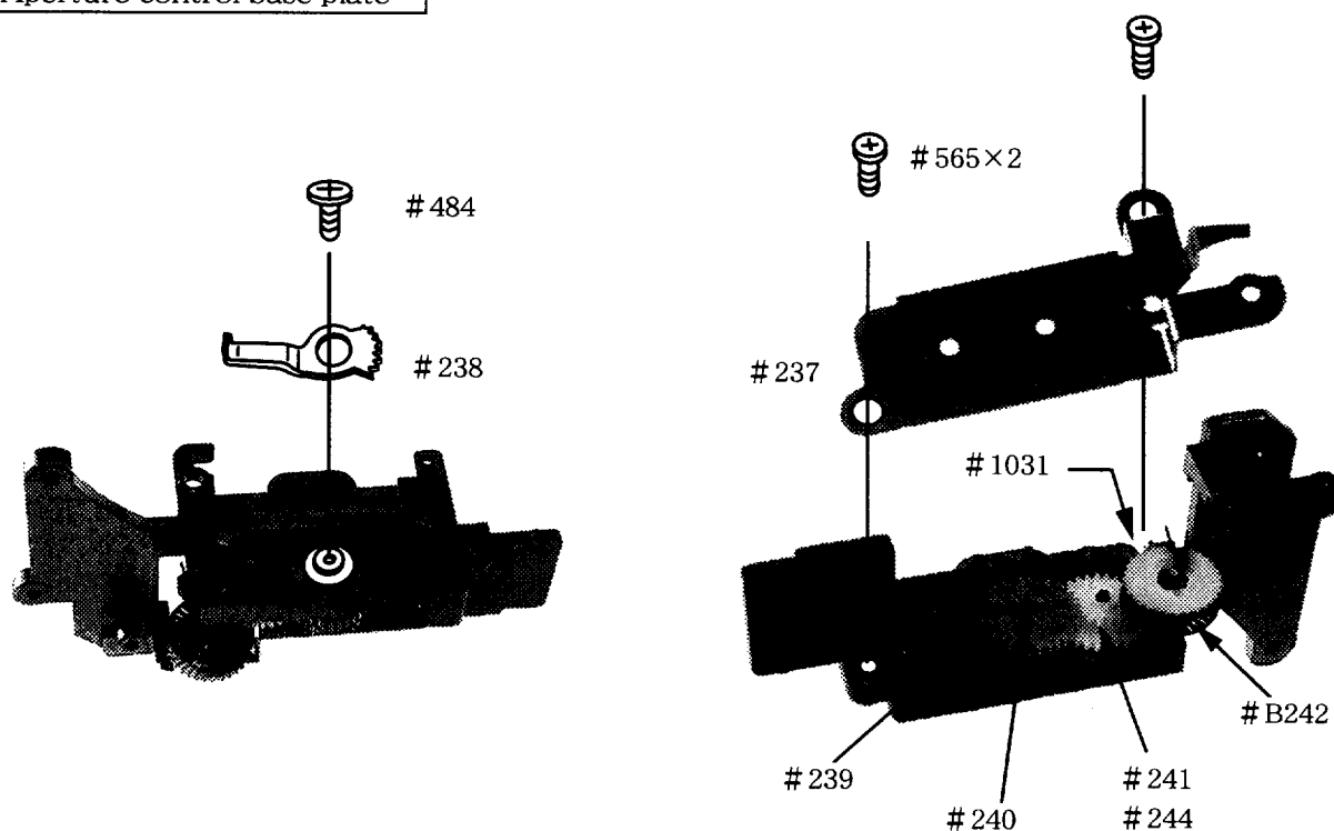
Aperture control base plate
