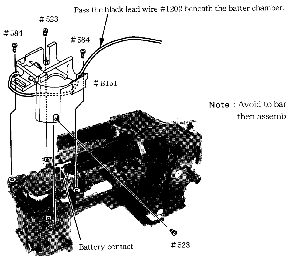
Battery chamber
