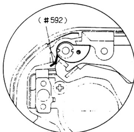
fig. 9-2 Spring #592
