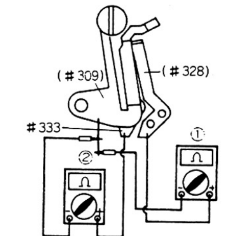
fig. 16-1 Connecting testers
