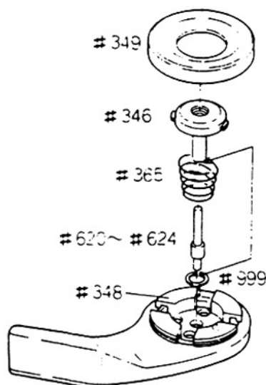
fig. 16-3 Shutter-release button
