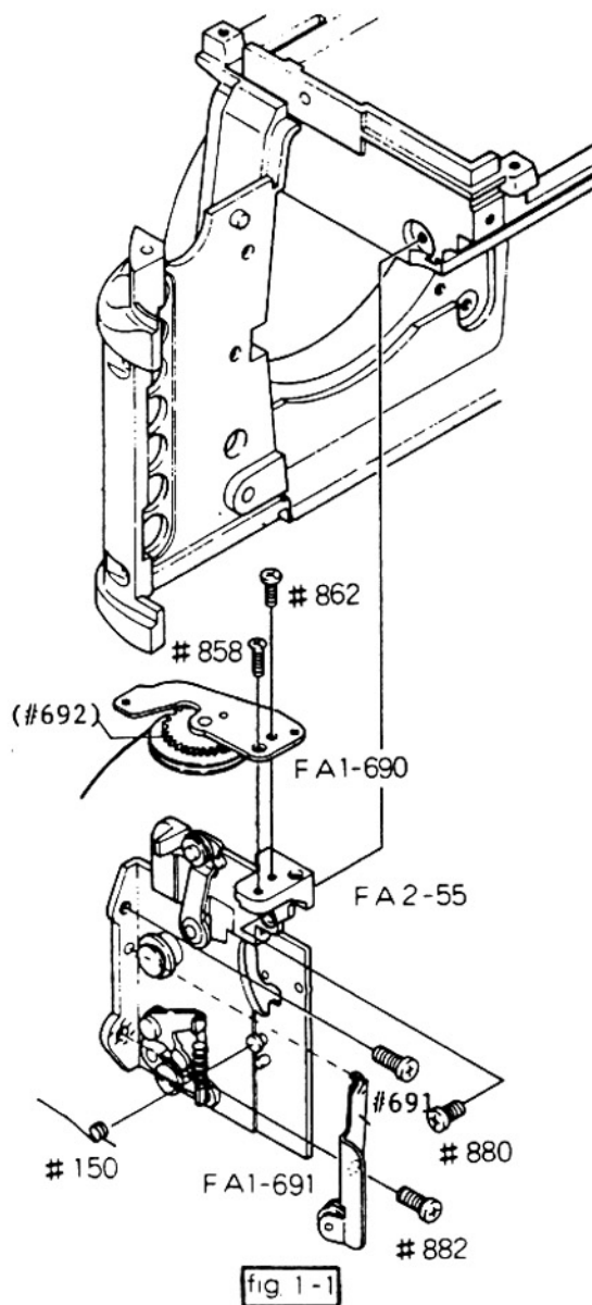
Front plate, rewind-side
