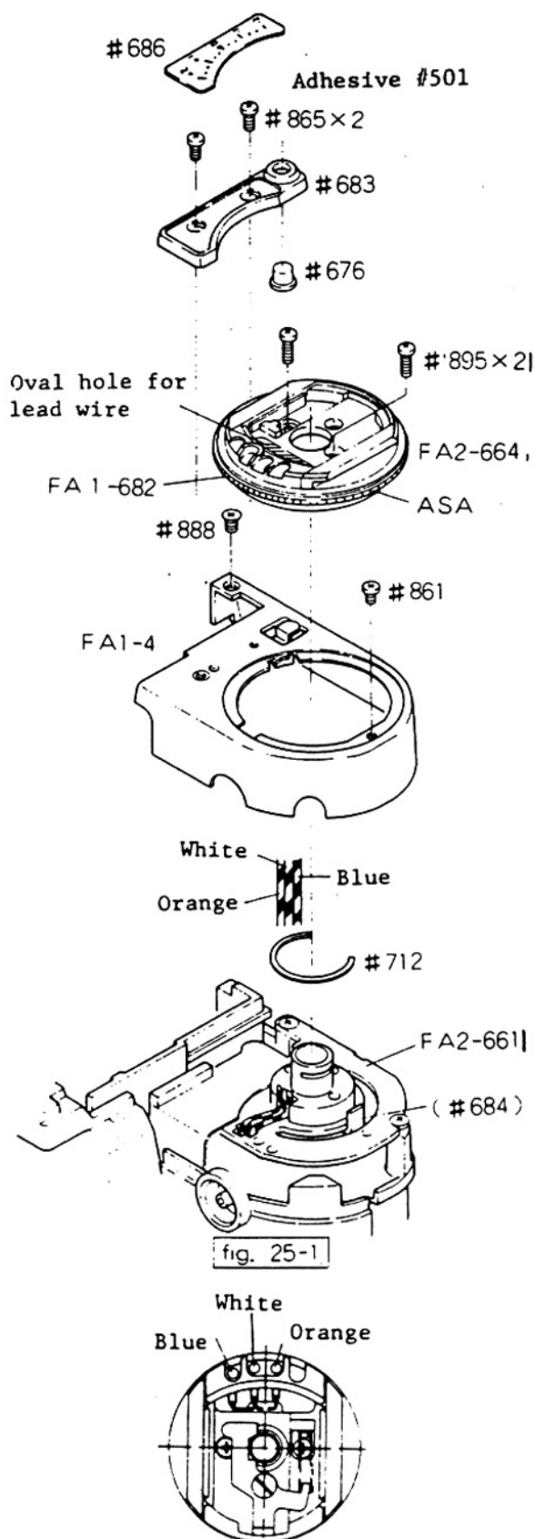
fig. 25-2 Lead Wire Soldering
