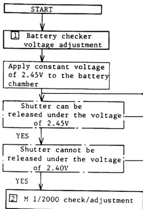
3-27-3 Flow-chart
