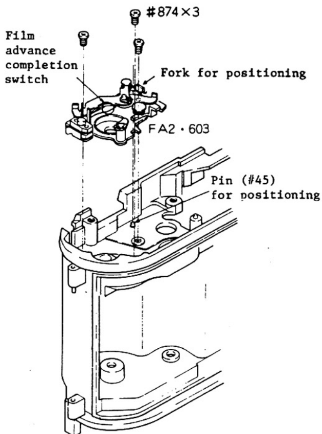
fig. 1-1 Body, wind side; with bottom up
