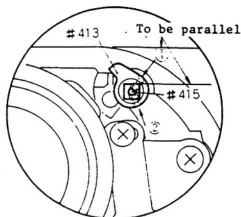
fig. 14-2 Coupler FA1-413
