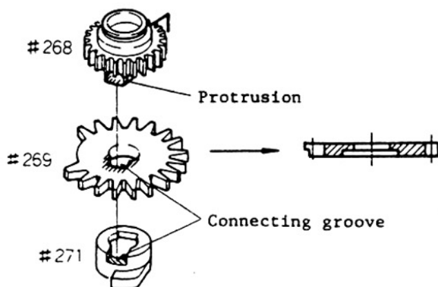
fig. 8-2 #269 installation
