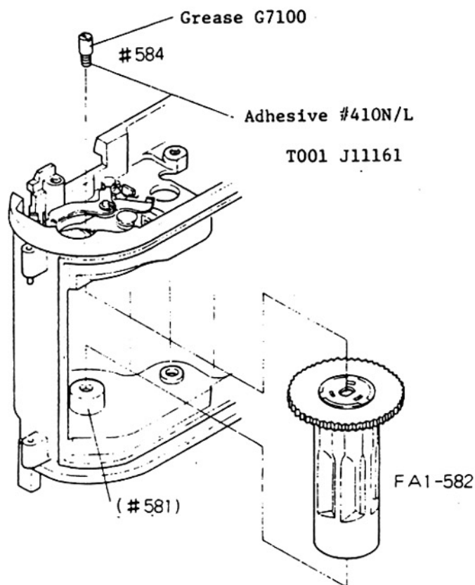
fig. 2-1, A2 Body, wind side; with bottom up
